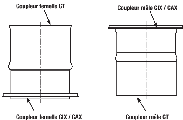
Figure 44 - Adaptateur CIX / CT, CT / CIX
